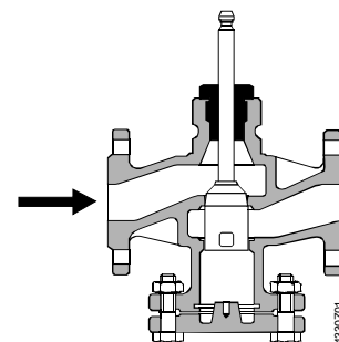
DN 50...100 closes against pressure
